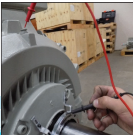
16) Check conductivity with multi meter between Electric motor casing and Earthring, the reading should be 1 ohms or less.
